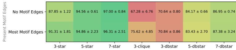
Figure 15: Comparison of the prediction accuracy of SEAM for different already present motif edges for the Power graph. h -hop = 1, learning rate = 0.002, number of epochs = 100, training dataset size = 100,000. The graph does not contain enough 5-cliques and 7-cliques due to its sparsity.
