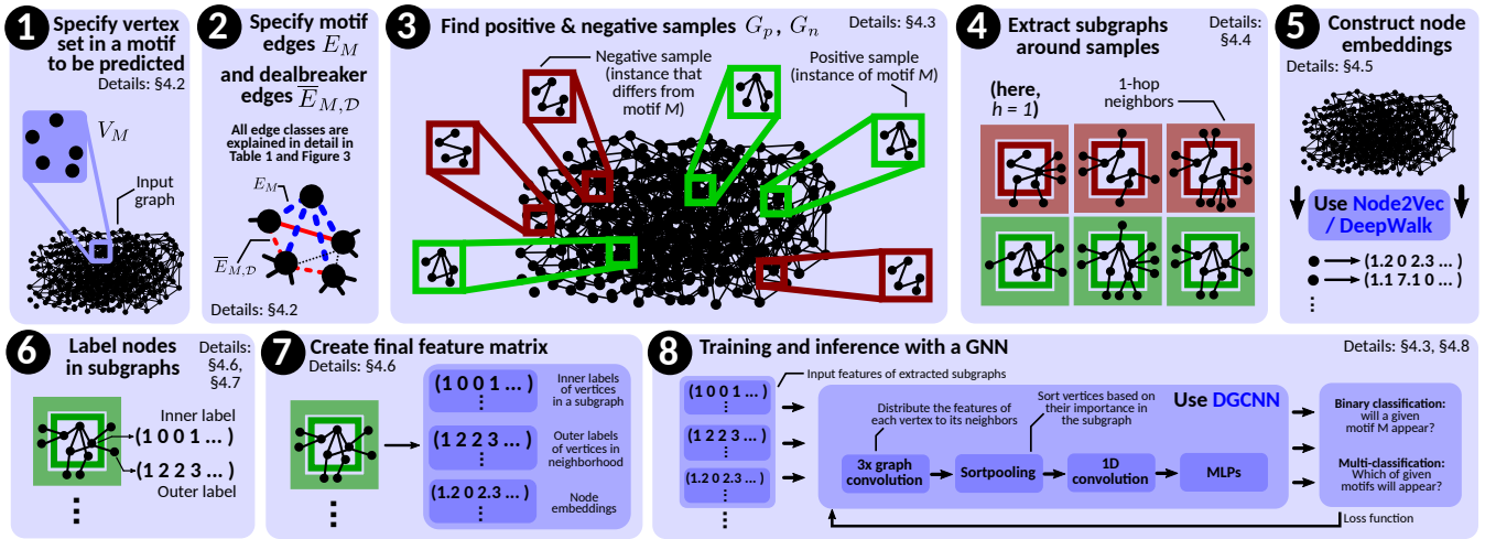
Figure 4: High-level overview of SEAM.
