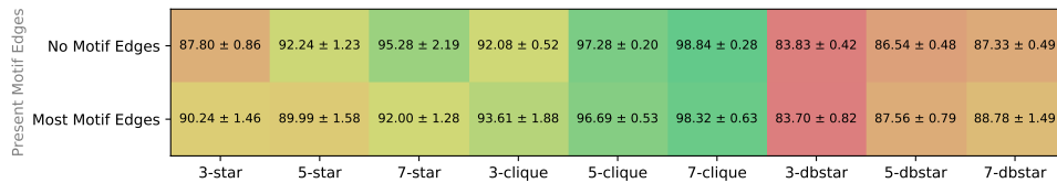
Figure 16: Comparison of the prediction accuracy of SEAM for different already present motif edges for the USAir graph. h -hop = 1, learning rate = 0.002, number of epochs = 100, training dataset size = 100,000.
