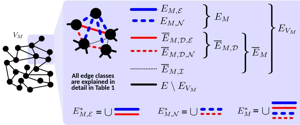
Figure 3: Illustration of edge types in motif prediction.
