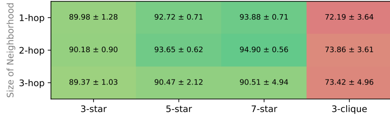
Figure 14: Comparison of different h -hop enclosing subgraphs used in SEAM, for the Power graph. Learning rate = 0.002, number of epochs = 100, training dataset size = 100,000. The graph does not contain enough 5-cliques and 7-cliques due to its sparsity.
