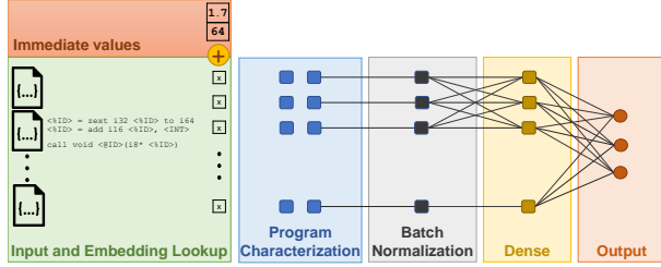
(a) concat_naive
