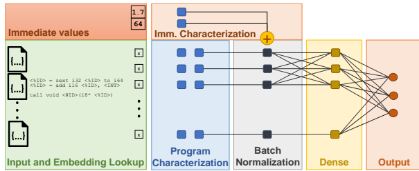
(c) extract_concat
