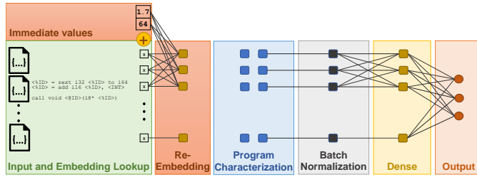
(b) concat_embed
