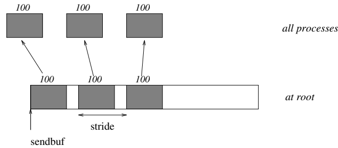
Figure 5.10: The root process scatters sets of 100 ints, moving by stride ints from sendbuf to send in the scatter.
